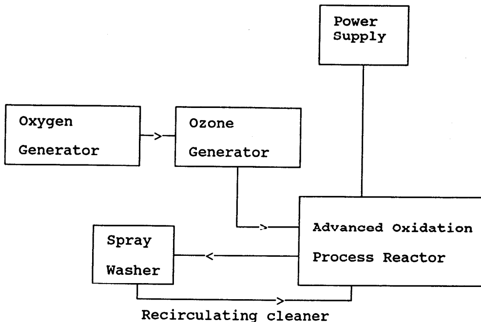
Figure 1. Process flow chart.
